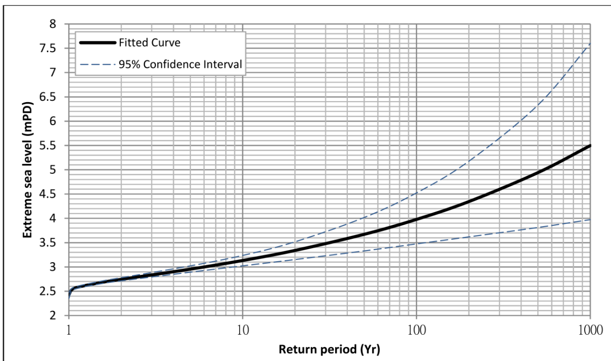
Figure D1 Extreme Sea Levels at Quarry Bay / North Point with pre-1954 records (1874-2019)
