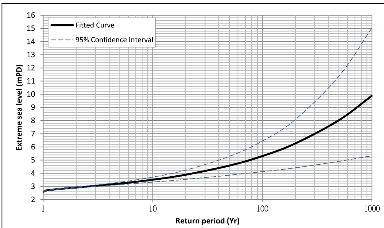
Figure D2 Extreme Sea Levels at Tai Po Kau with pre-1954 records (1874-2019)
