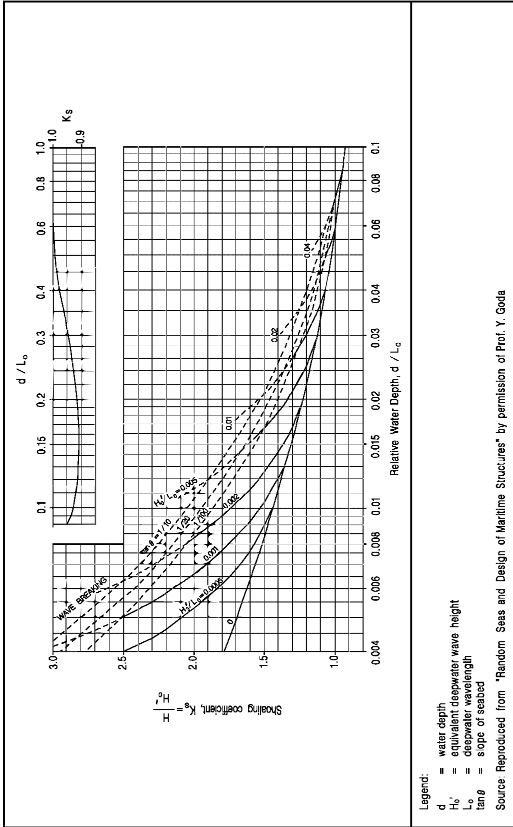
Figure A1 – Diagram of Nonlinear Wave Shoaling
